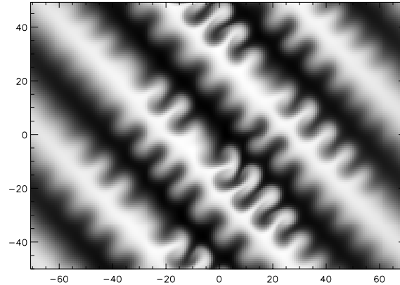
Figure 1. Grey scale plot of the slightly nonlinear state of the secondary instability of a strong drift wave from a numerical simulation of the drift wave and streamer equation including all harmonics. The length units of the plot are \rho_s (as throughout the paper), the wavenumber of the primary mode is 0.089, its peak velocity (in the region of maximum gradient) is 10.7v_d , the wavenumber of the perturbation is measured to be 0.64.
